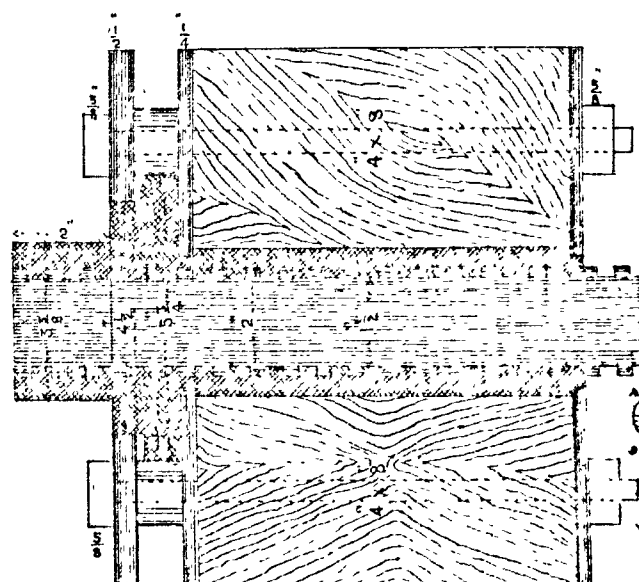
SECTION ON E.E.
