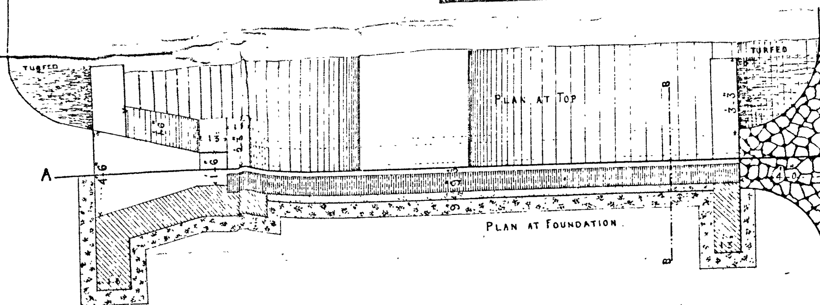
PLAN OF A BARREL SLUDGE
