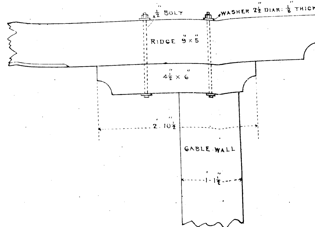
DETAIL OF RIDGE OVER GABLE WALL 1/12 ACTUAL SIZE.
