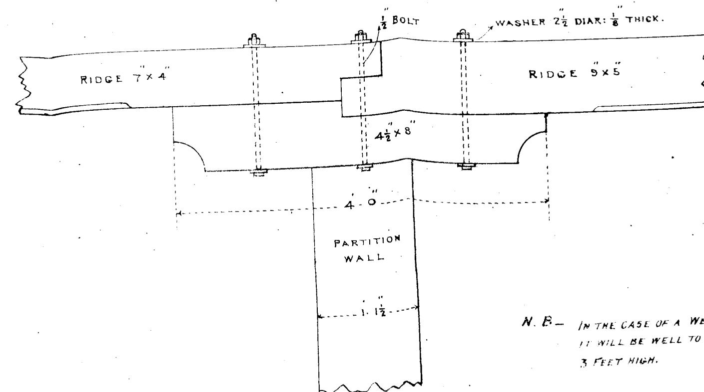
DETAIL OF RIDGE OVER PARTITION WALL. 1/12 ACTUAL SIZE.
