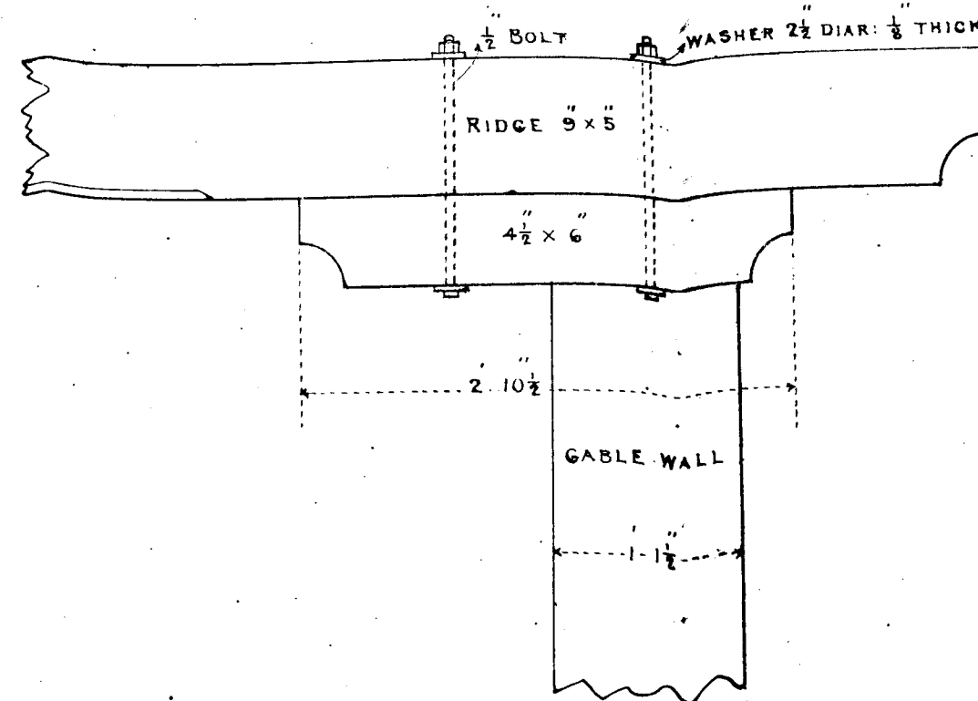
DETAIL OF RIDGE OVER GABLE WALL \frac{1}{12} ACTUAL SIZE.
