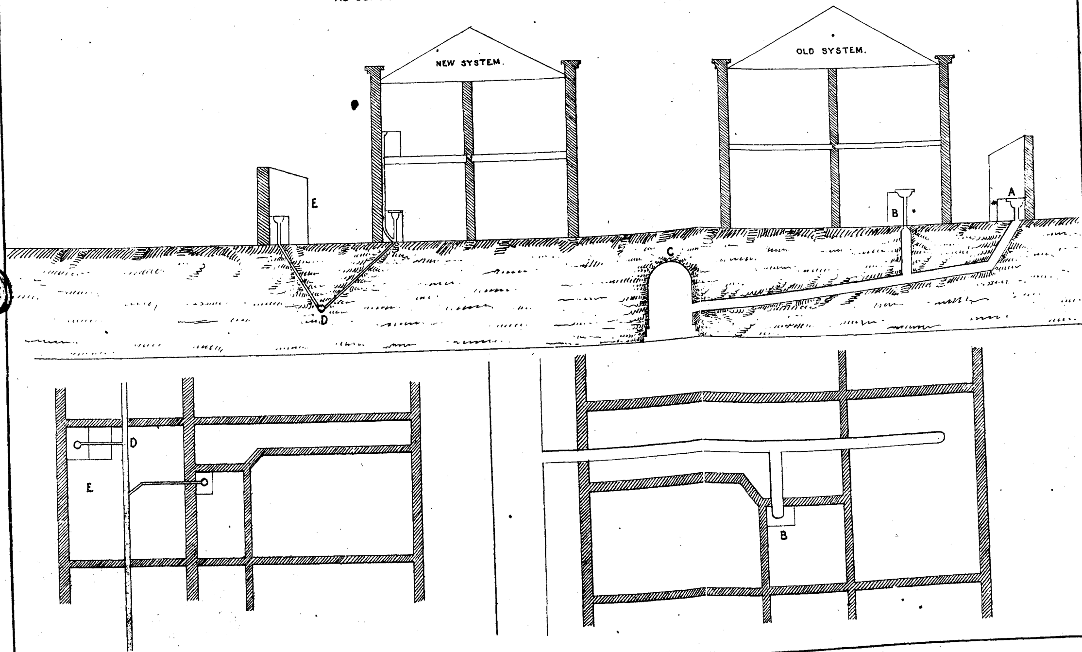
PLANS AND TRANSVERSE SECTIONS SHEWING THE RELATIVE FRICTIONAL AREAS OF THE SELF CLEANSING NEW SYSTEM AS COMPARED WITH THE OLD SYSTEM OF HOUSE DRAINS IN LONDON.
