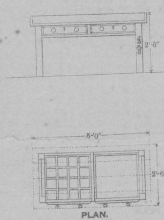
WATCH MAKERS' BENCH. ELEVATION.
