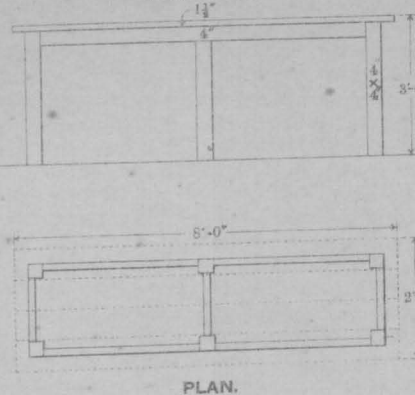
SHOEMAKERS' BENCH. ELEVATION.
