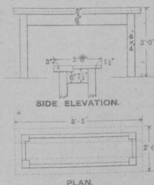
TINSMITHS' BENCH. ELEVATION.
