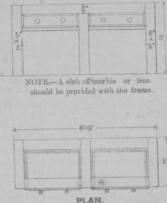
IMPOSING TABLE. ELEVATION.
