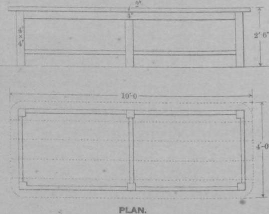
TAILORS' BENCH. ELEVATION.
