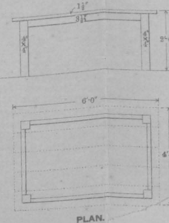
TAILORS' TABLE. ELEVATION.
