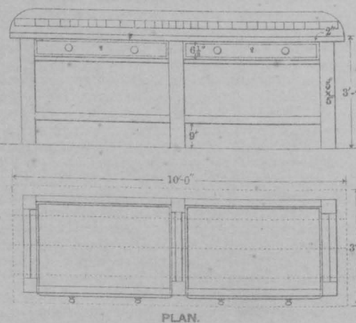
COLLAR MAKERS' TABLE. ELEVATION.
