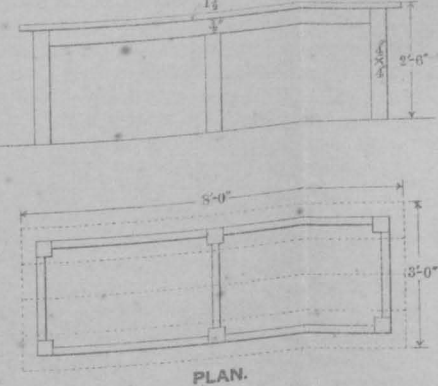
PAINTERS' TABLE. ELEVATION.
