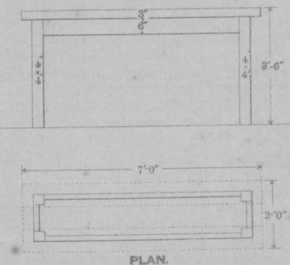
TURNERS' BENCH ELEVATION.
