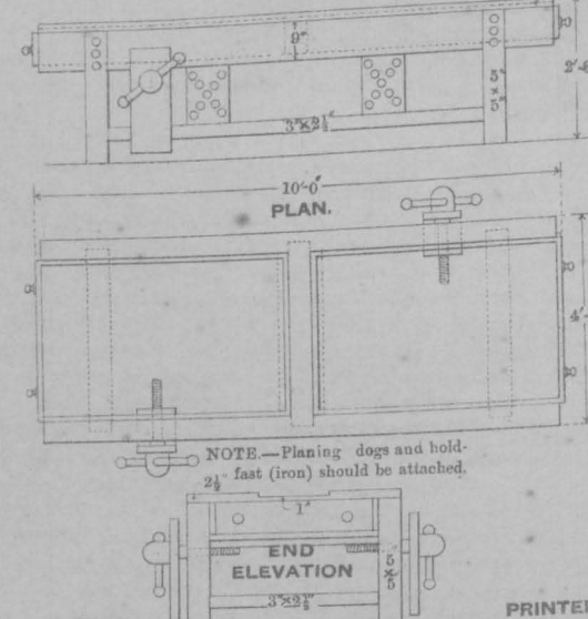
COMPOSING FRAME. FRONT ELEVATION.
