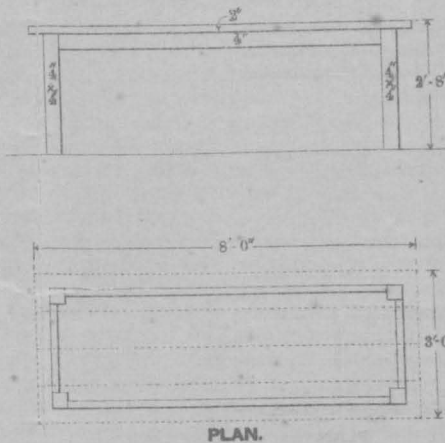
BOOKBINDERS' BENCH. ELEVATION.
