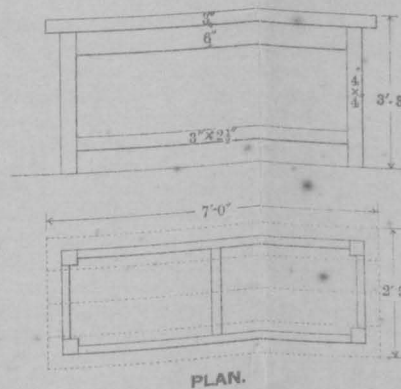
BLACKSMITHS' TABLE. ELEVATION.
