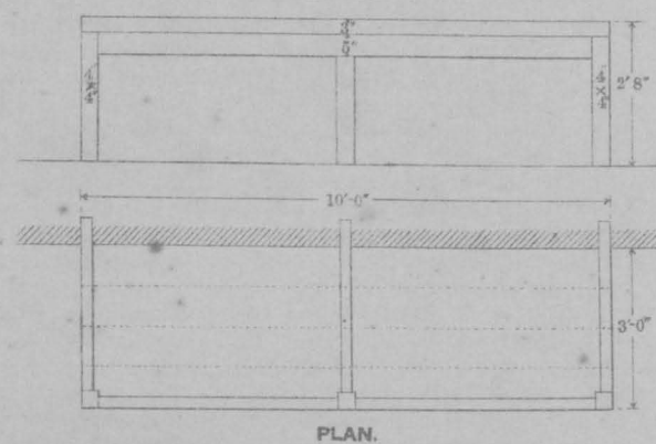
BLACKSMITHS' BENCH. ELEVATION.
