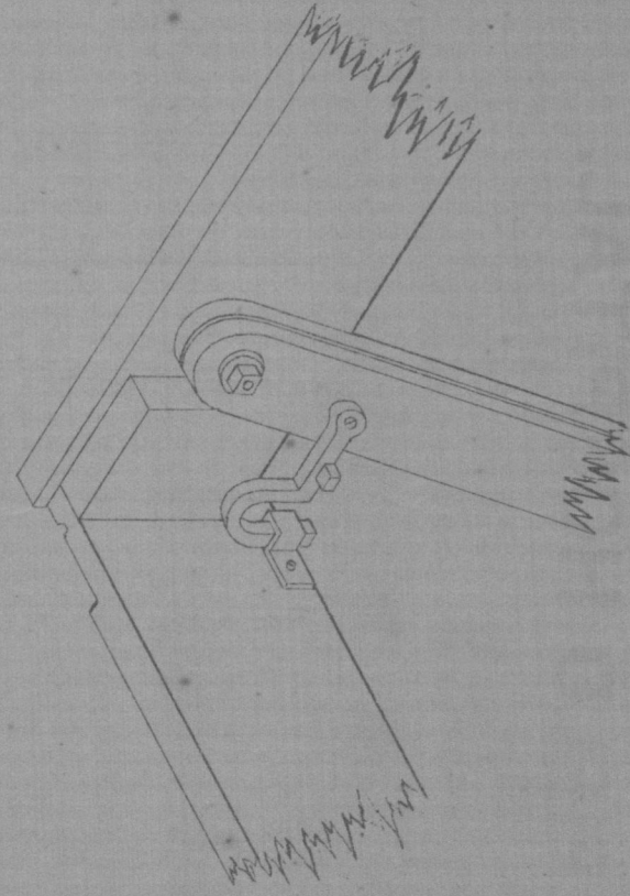
INSIDE VIEW OF CORNER OF TABLE TO SHOW HOOK AND CATCH WHEN TABLE IS OPEN.
