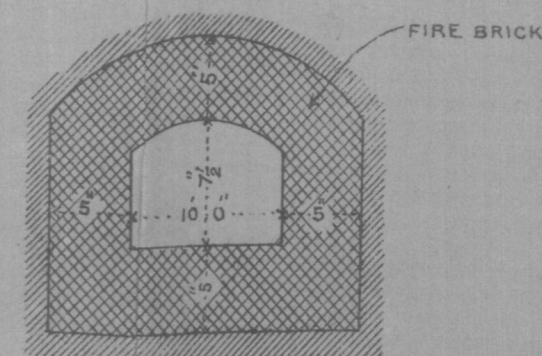
SECTION OF FLUE ON .S. T. (SEE PLAN ON .O. N.)
