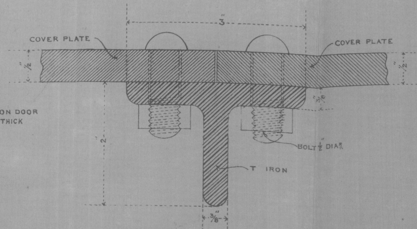
SECTION OF FLUE ON .S. T. (SEE PLAN ON .O. N.)
