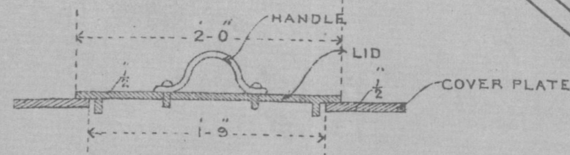
SECTION OF LID TO COVER HOLES.
