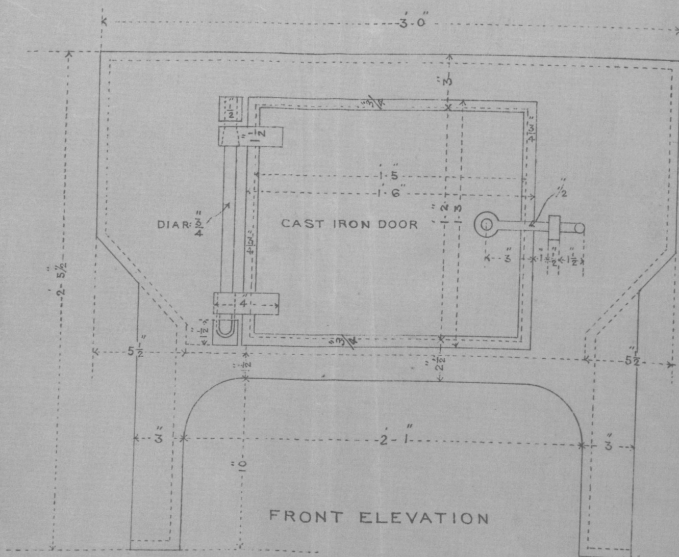
DETAILS OF CAST IRON DOOR AND FRAME.
