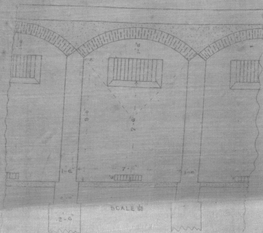
SECTION
