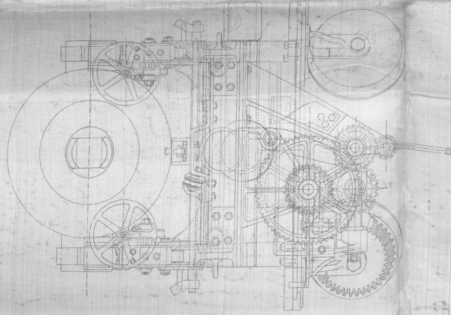
REAR ELEVATION
