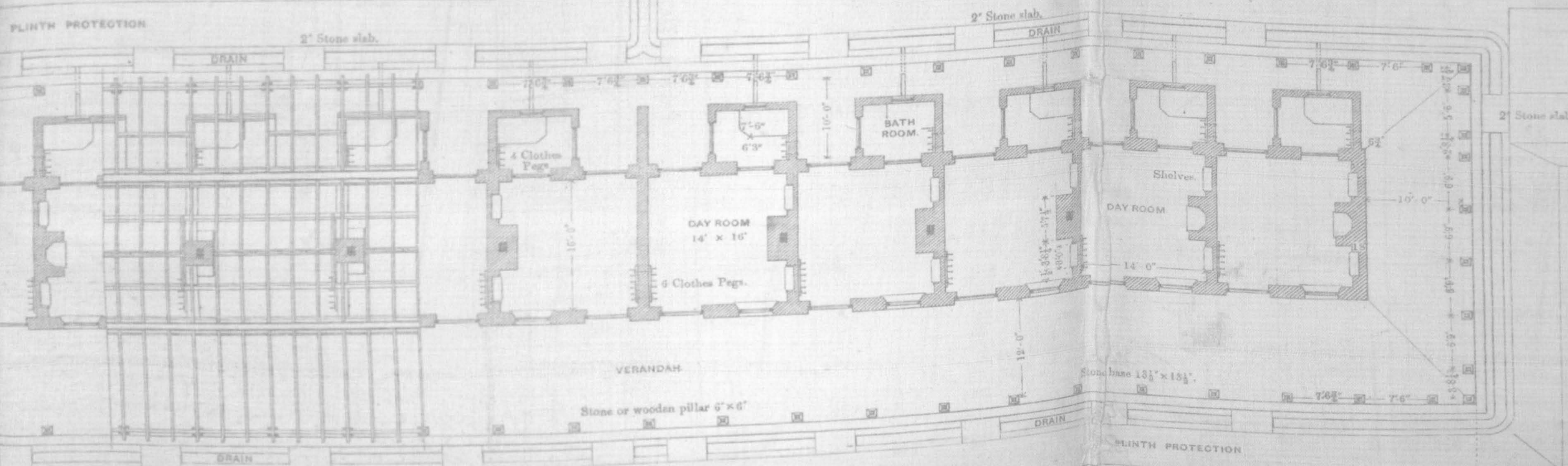
PLAN OF 10 CLASS I QUARTERS. PLINTH AREA EXCLUSIVE OF STEPS AND DRAIN = 7,449 S. FT.
