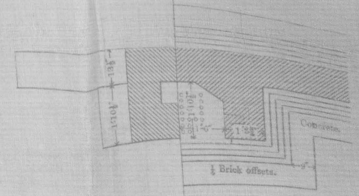
SECTION OF FIREPLACE CLASS I QUARTERS. FIG. VIII.
