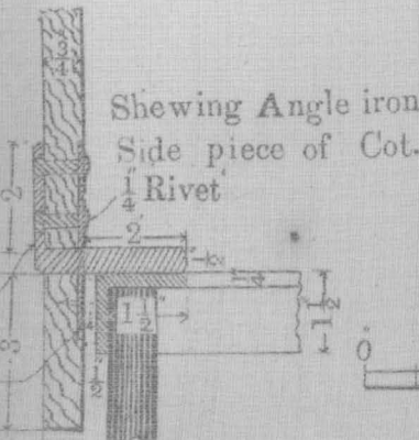
SECTION ON O. P
