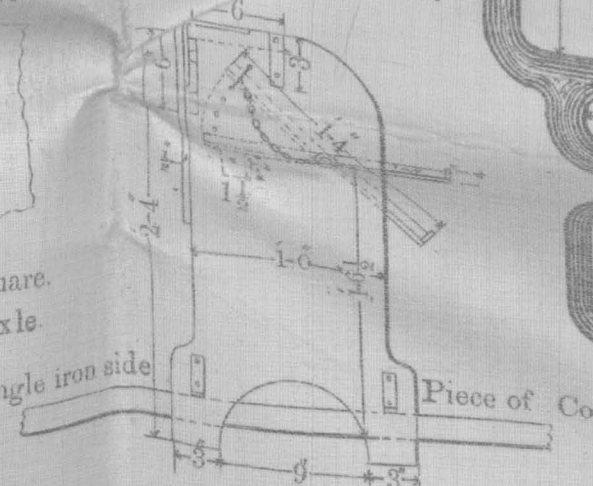
FIG VII SIDE ELEVATION ON E. F
