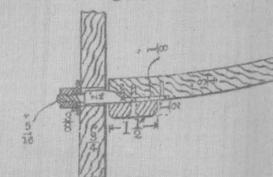
FIG V LOWER PLAN
