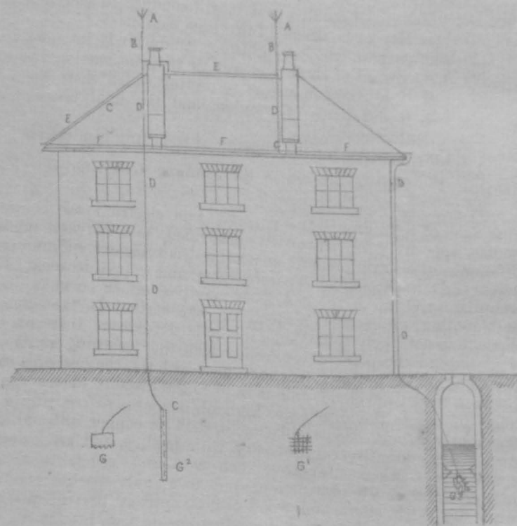
INDEX SKETCH OF LIGHTNING CONDUCTOR, ILLUSTRATING THE TERMS EMPLOYED IN THE REPORT.
