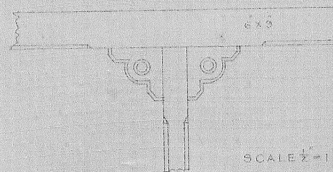
DETAILS FOR VERANDAH
