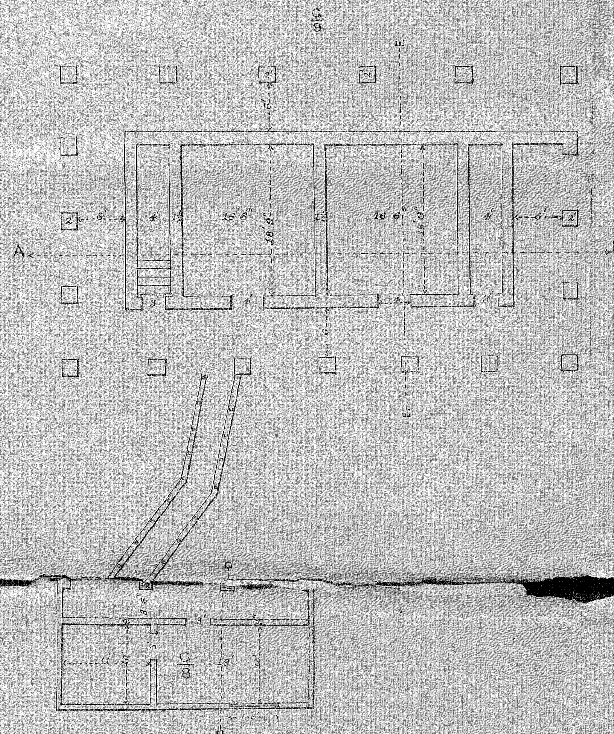
PLAN OF LOWER PORTION
