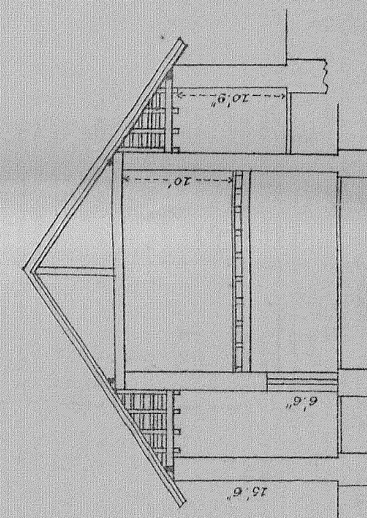
SECTION E.F.
