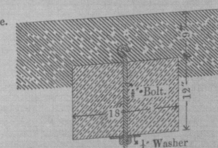
SECTION THROUGH STONE BLOCK AT END OF GUY ROD.
