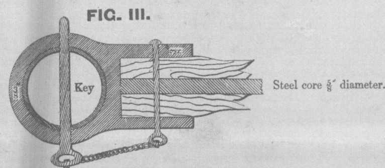
SECTION THROUGH SOCKET AND GUIDE.
