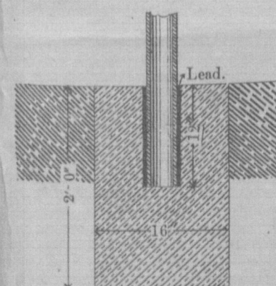
SECTION THROUGH STONE BLOCK AT FOOT OF UPRIGHT.
