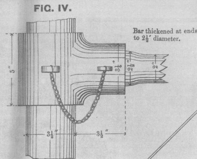
ELEVATION OF SOCKET AND GUIDE.
