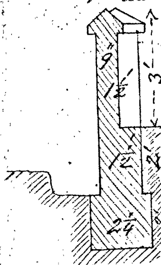
Section of East wall
