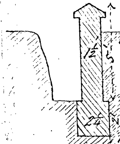
Section of Southern wall.
