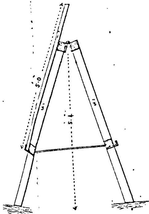
Section of Black board
