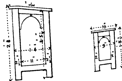
Writing Desk & Form 12 Feet long
