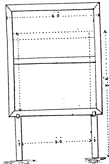
Elevation of Black board
