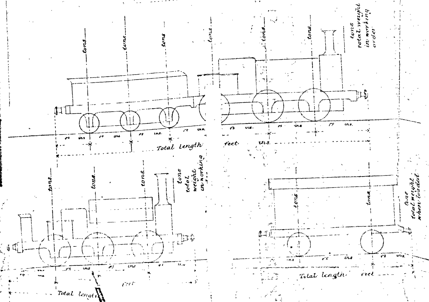
DIAGRAMS SHEWING DIMENSIONS AND LOADS OF ENGINES AND WAGONS IN USE ON THE RAILWAY.
