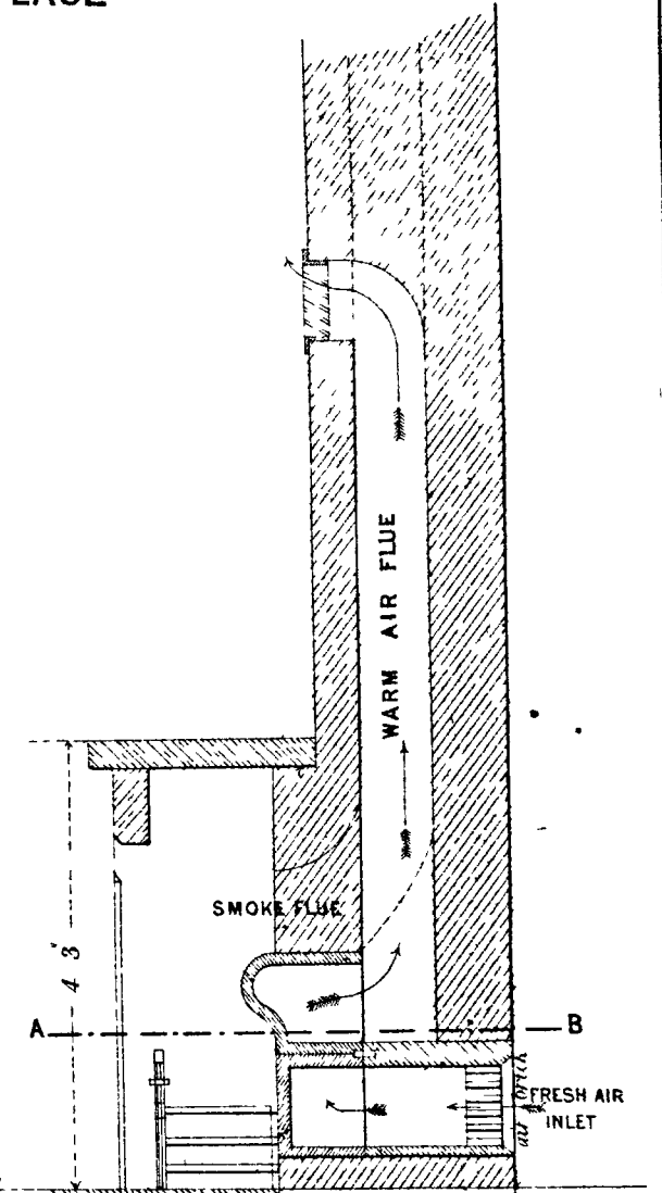
SECTION C D ON PLAN
