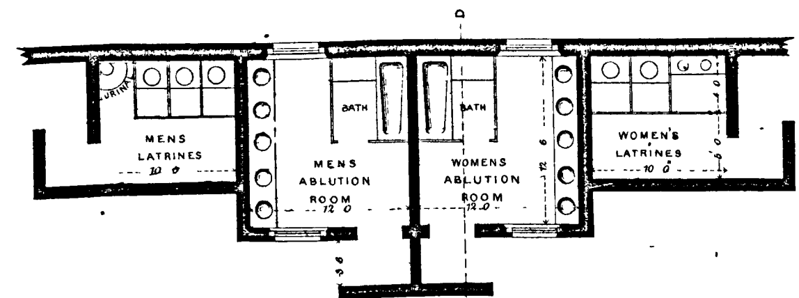
PLAN
