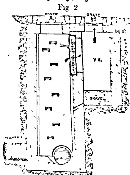
Manhole and Ventilating Shaft.
