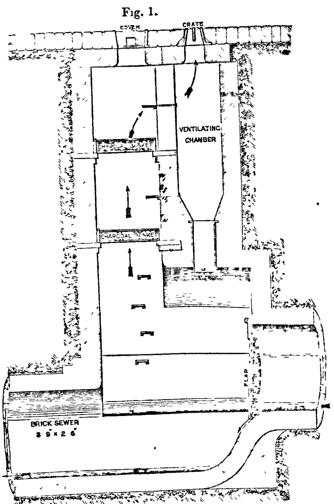
Manhole, Tumbling Bay, and Double Ventilating Arrangement
