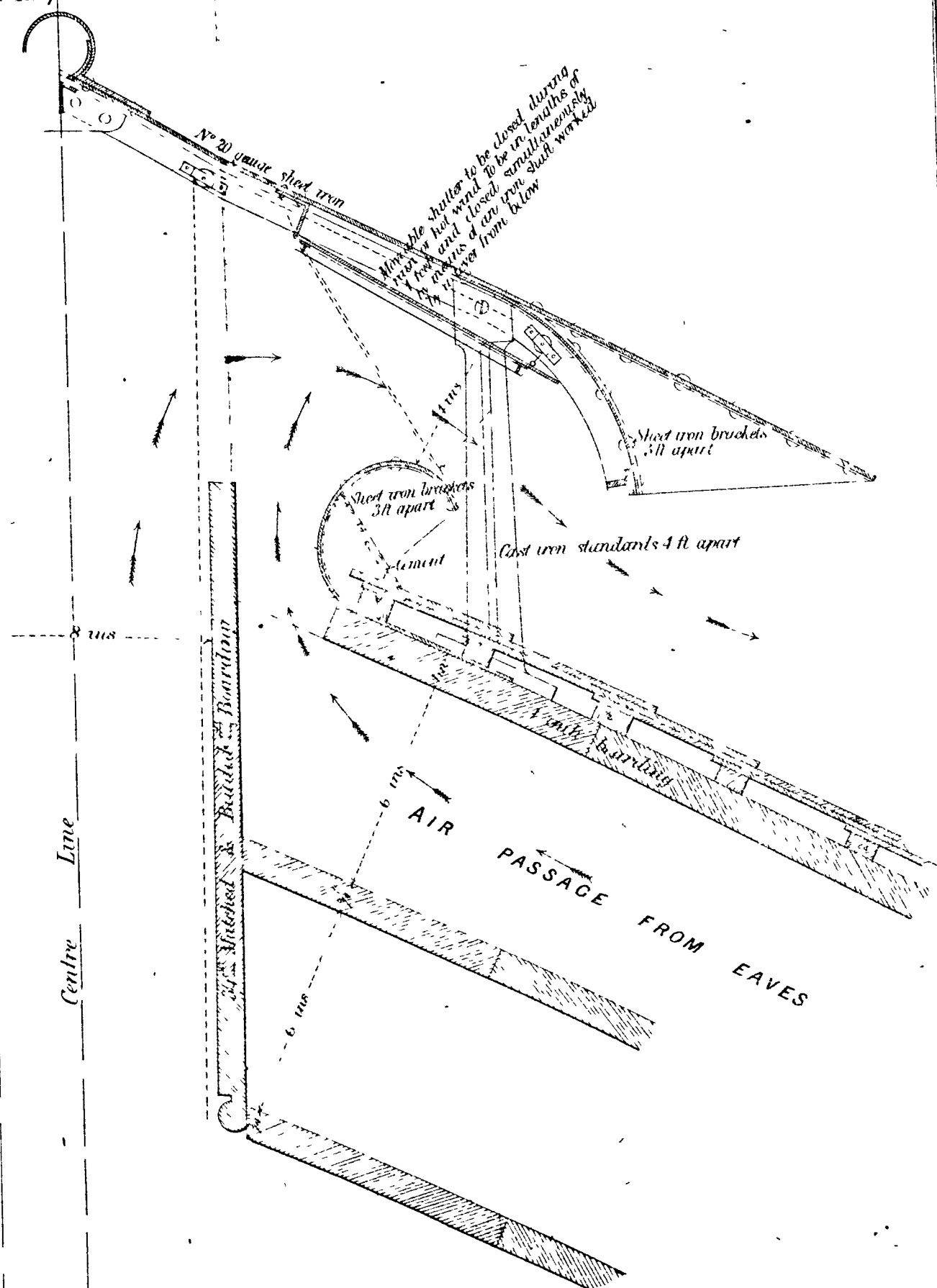
SECTION OF CONTINUOUS VENTILATOR ON ROOF
