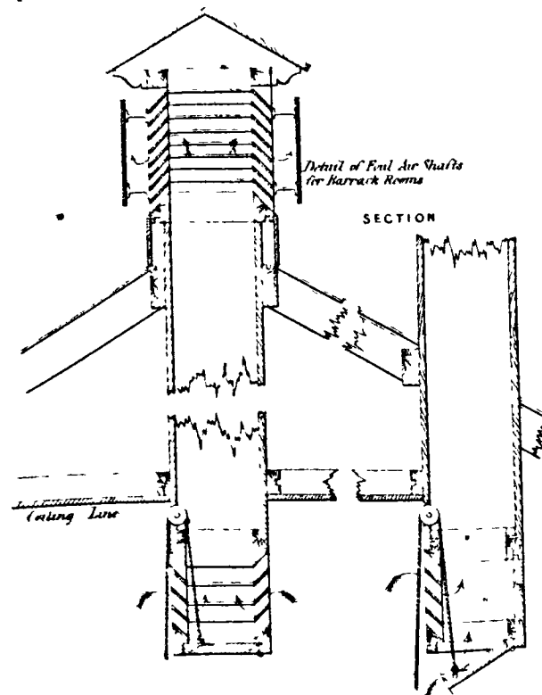
ELEVATION OF LOWER END OF SHAFT
