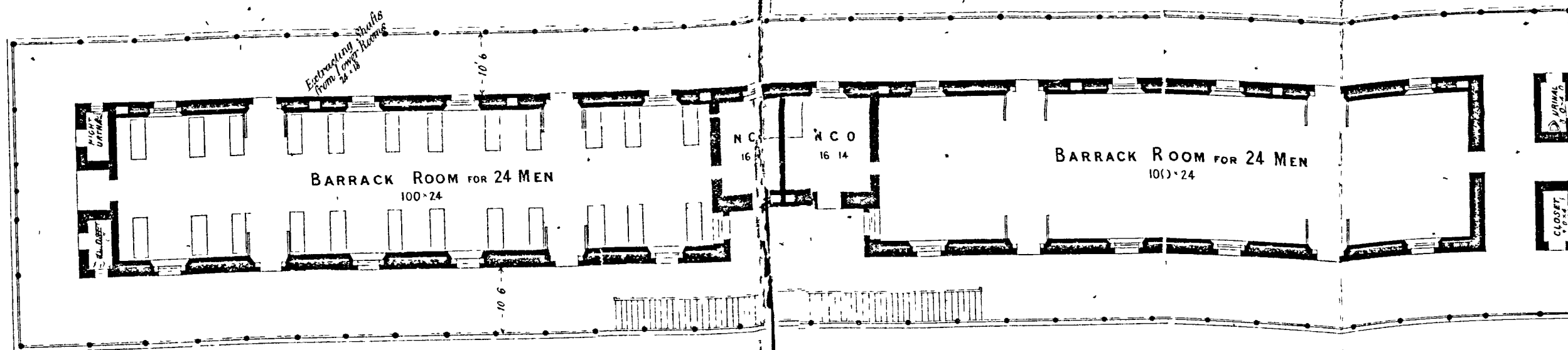
PLAN OF UPPER FLOOR
