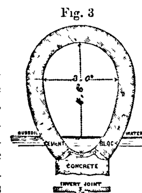
Main Outlet Sewer, West Ham
