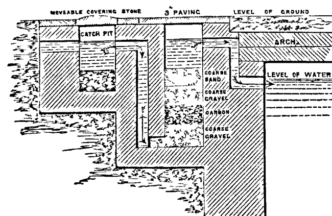
FIG 6—DETAIL OF SINGLE FILTER FOR RAIN-WATER TANK Section on Line A B.
