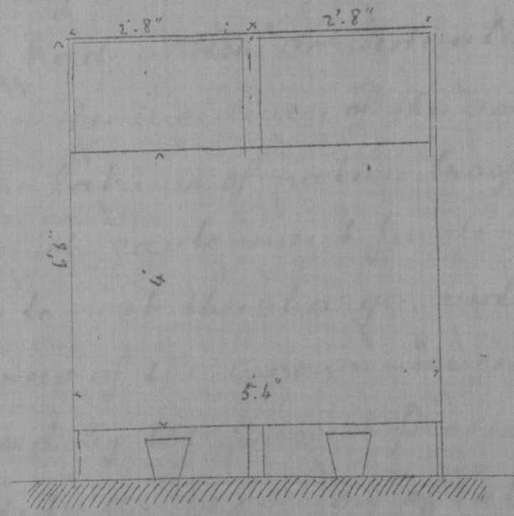
BACK ELEVATION
