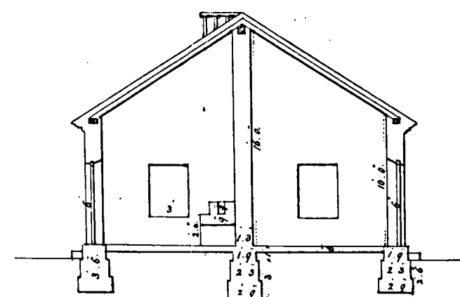
Section thro' C. D.
