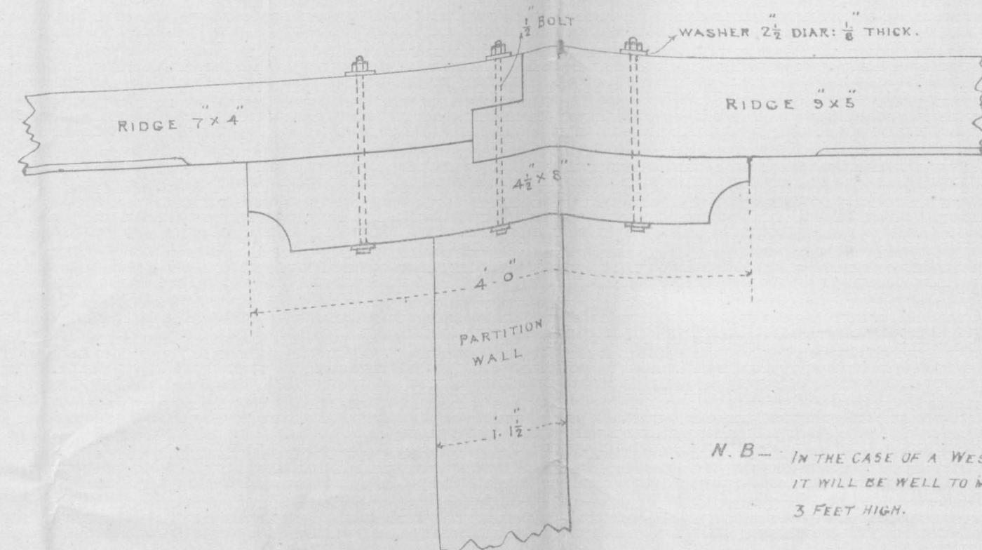
DETAIL OF RIDGE OVER PARTITION WALL. 1/2 ACTUAL SIZE.
