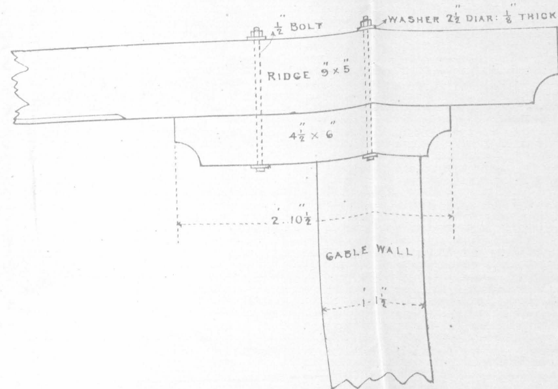
DETAIL OF RIDGE OVER GABLE WALL. 1/2 ACTUAL SIZE.
