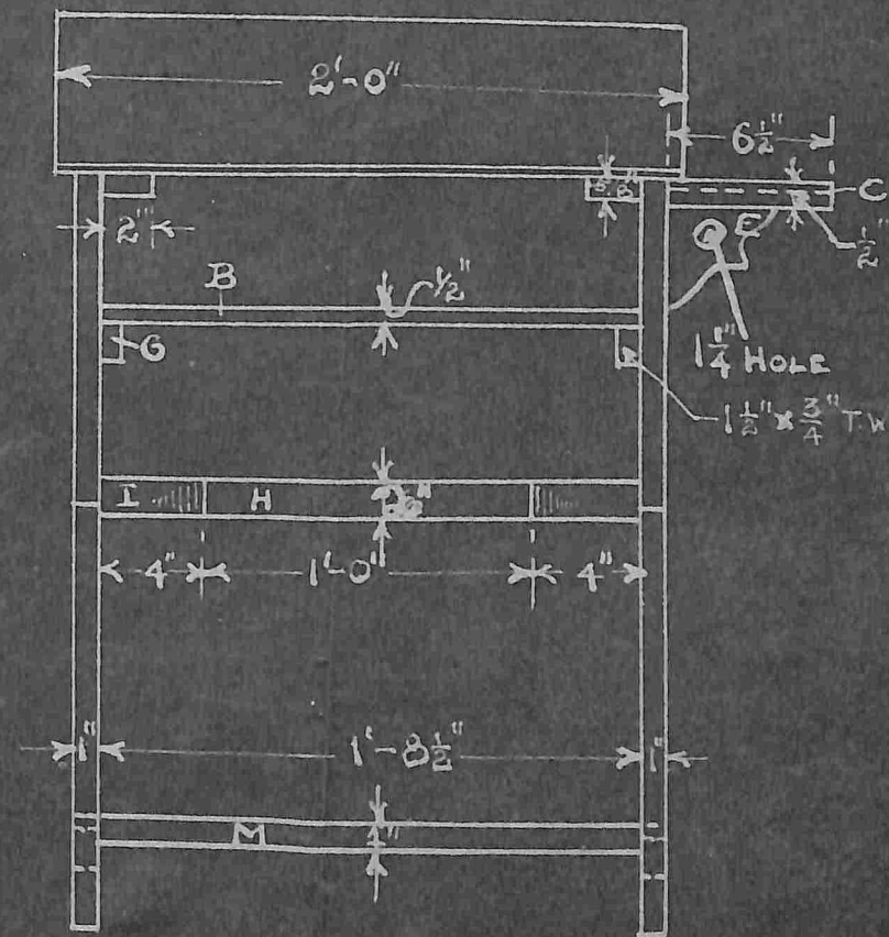
FRONT VIEW
