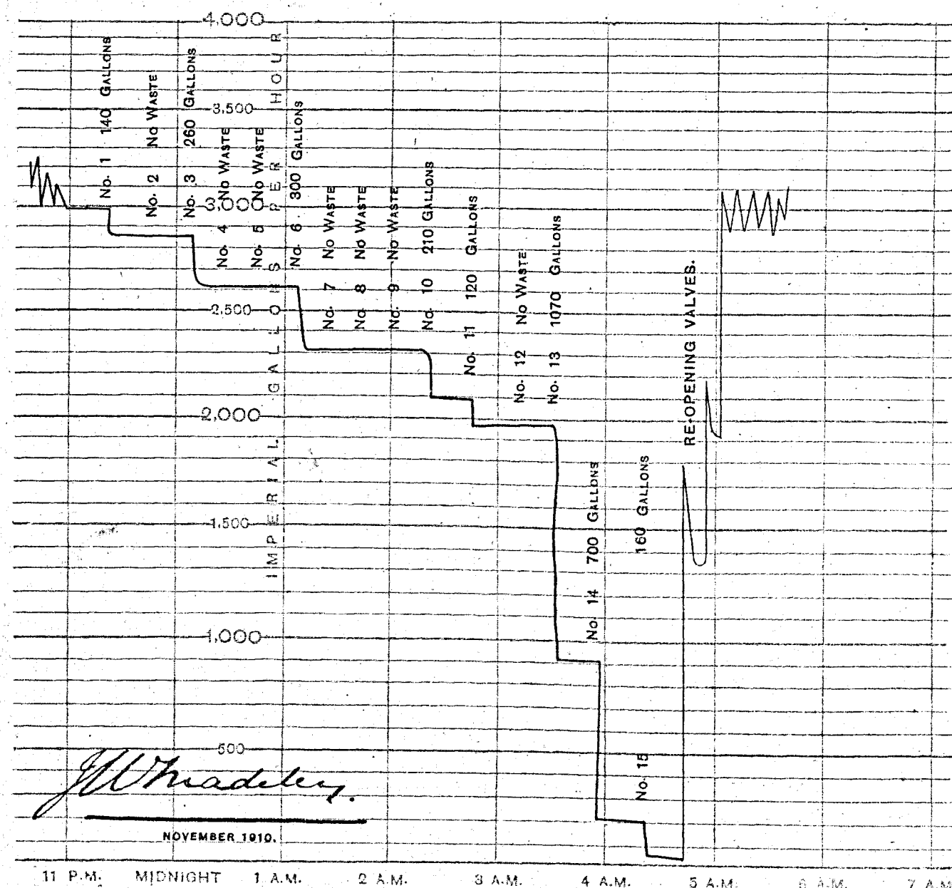
FIG. 2. PART OF IMAGINARY DIAGRAM—FULL SIZE—SHEWING RECORD OF A NIGHT INSPECTION AND THE EFFECT OF CLOSING DIFFERENT VALVES.
