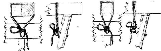
Rack lashing
