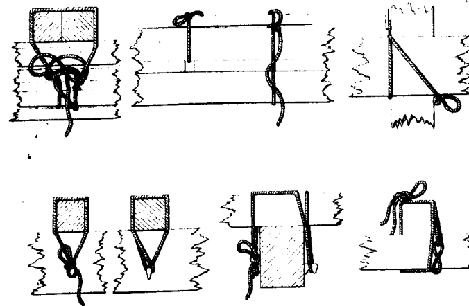
Rack lashing
