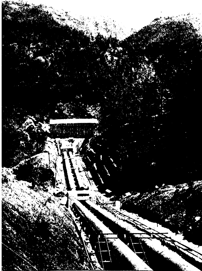
KUNDAH HYDRO-ELECTRIC SCHEME Penstocks and Rear view of Power-House I.
