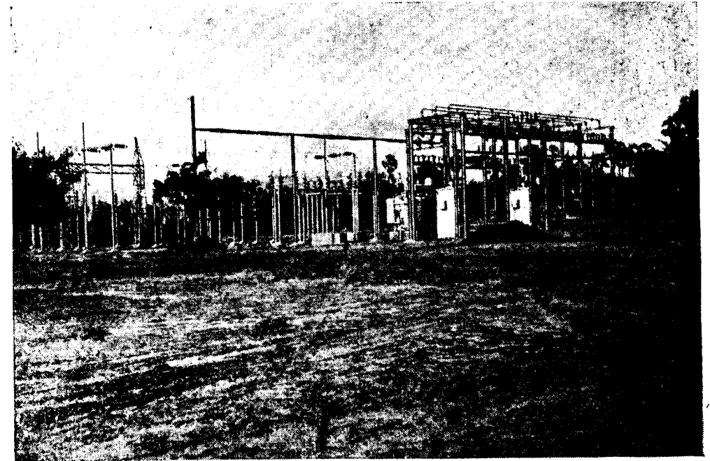
PAPANASAM ELECTRICITY SYSTEM. Nagercoil 66/11 K.V. Sub-station.
