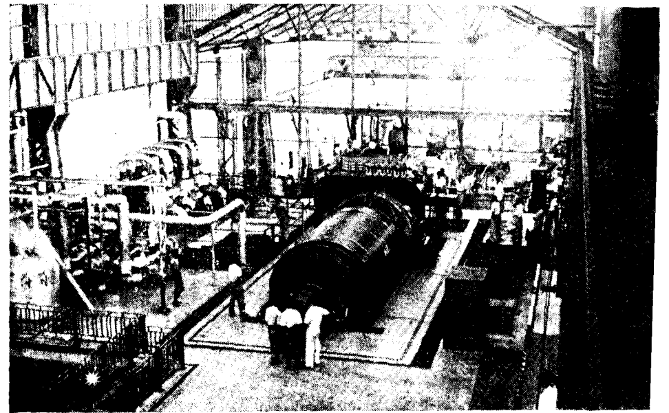
BASIN BRIDGE POWER STATION. View of T.A. set No. 3.
