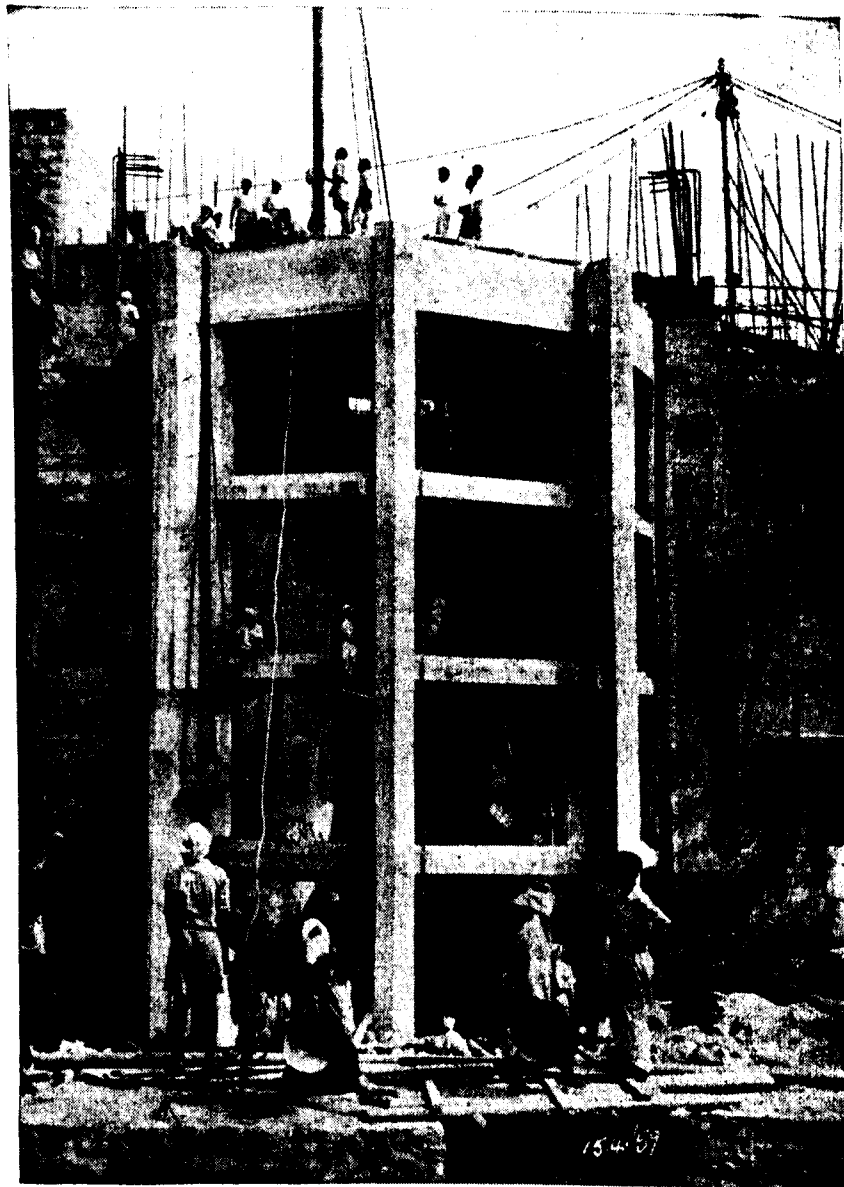
KUNDAH HYDRO ELECTRIC SCHEME. D/1. AVALANCHE DAM. (A view of trash rack piers for Scour vent as seen from upstream side.)
