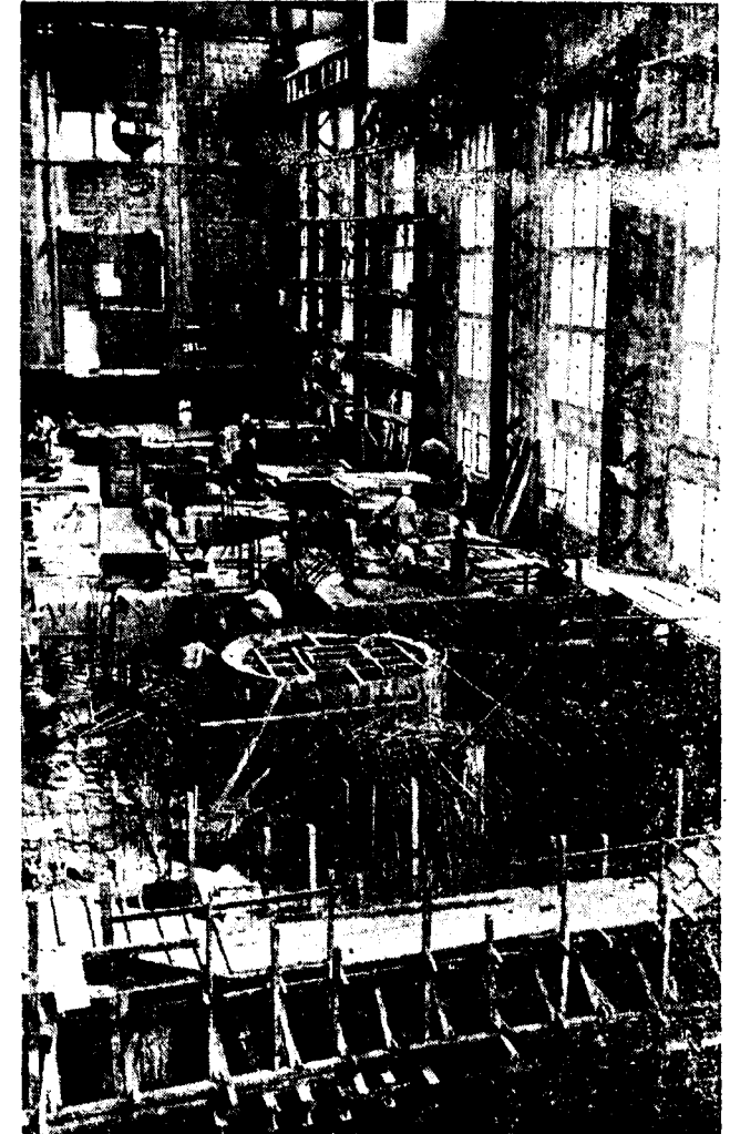
PERIYAR H. E. S.—Inside View of the Power House Reinforcement net for No. 3 Generator slab after I stage concreting.
