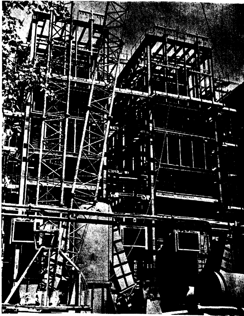
BASIN BRIDGE 'C' STATION 150,000 LBS./PER HOUR BOILERS UNDER ERECTION.
