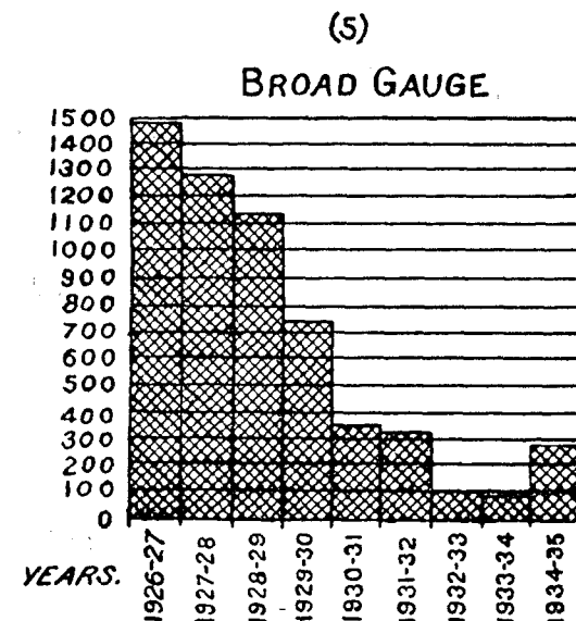
Number of coaching stock units provided in the rolling stock programme.
