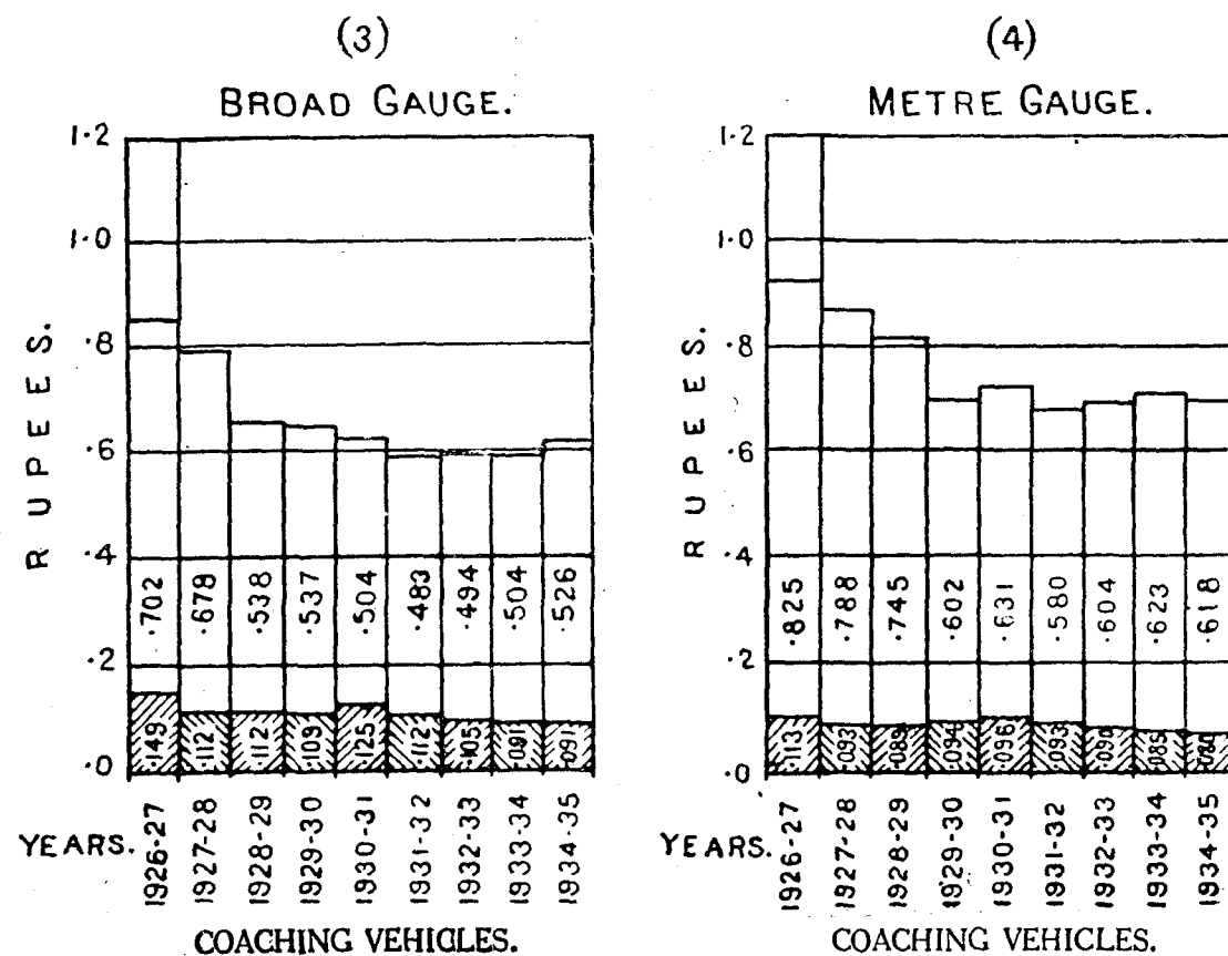
COST OF MAINTENANCE AND OPERATION OF CARRIAGE AND WAGON STOCK PER 1,000 GROSS TON MILES.
