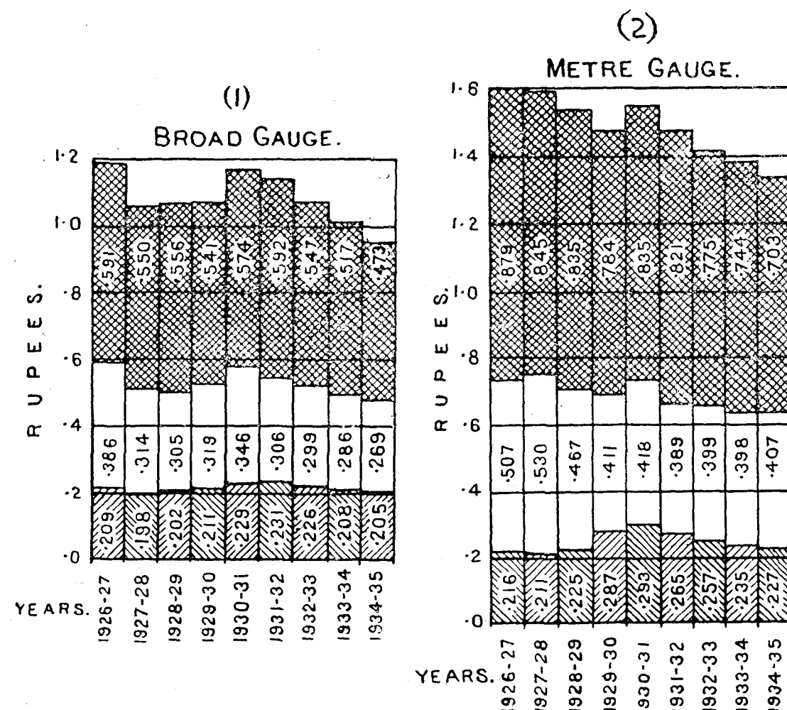
COST OF MAINTENANCE AND OPERATION OF CARRIAGE AND WAGON STOCK PER 1,000 GROSS TON MILES.
