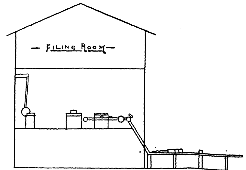
CROSS SECTION THROUGH TRIM SAW. ROLLS, EQUALIZER, SKIDS & SKID SORTING TABLE.
