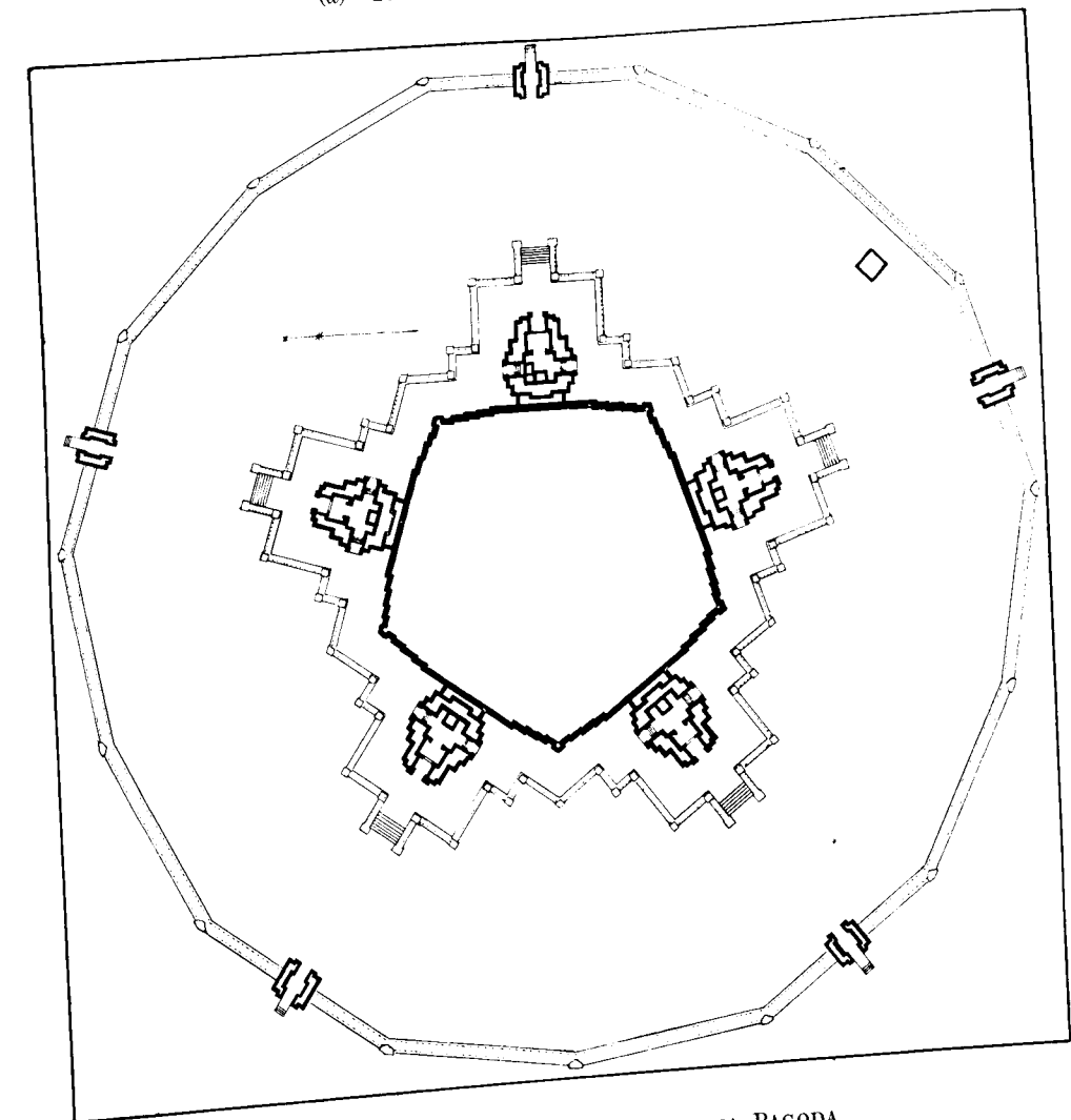
(b) PAGAN: PLAN OF DHAMMAYAZIKA PAGODA.
