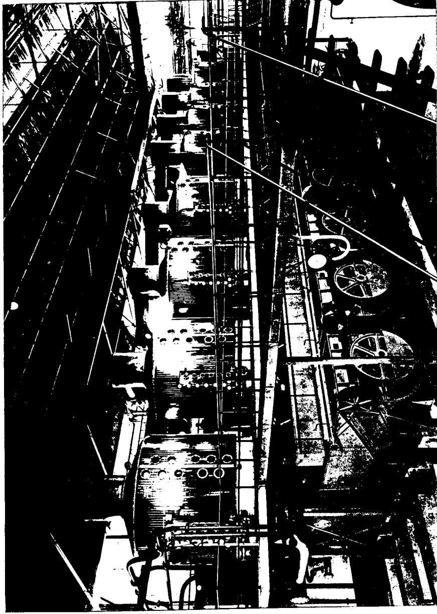
(8). View of Tiepiping Sugar Factory, Java. Vacuum Pans and Evaporators, with Crystallisers below. (Reproduced by courtesy of Messrs. McNeill and Co., Semarang.)
