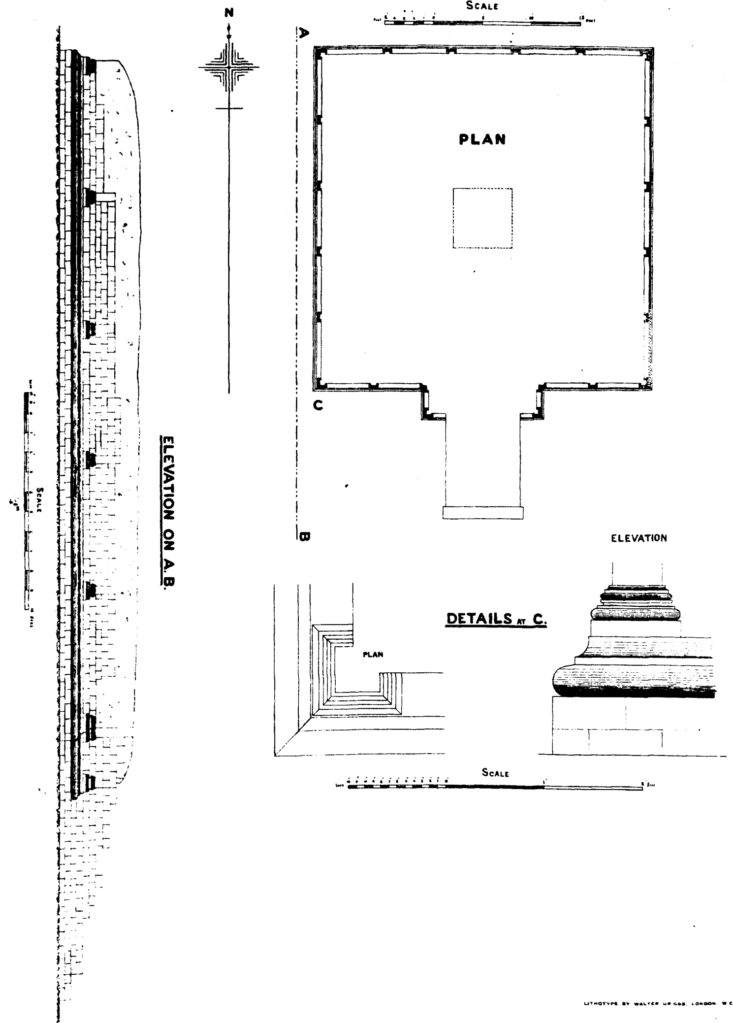
PLAN AND ELEVATION OF STUPA A. JANDIAL.
