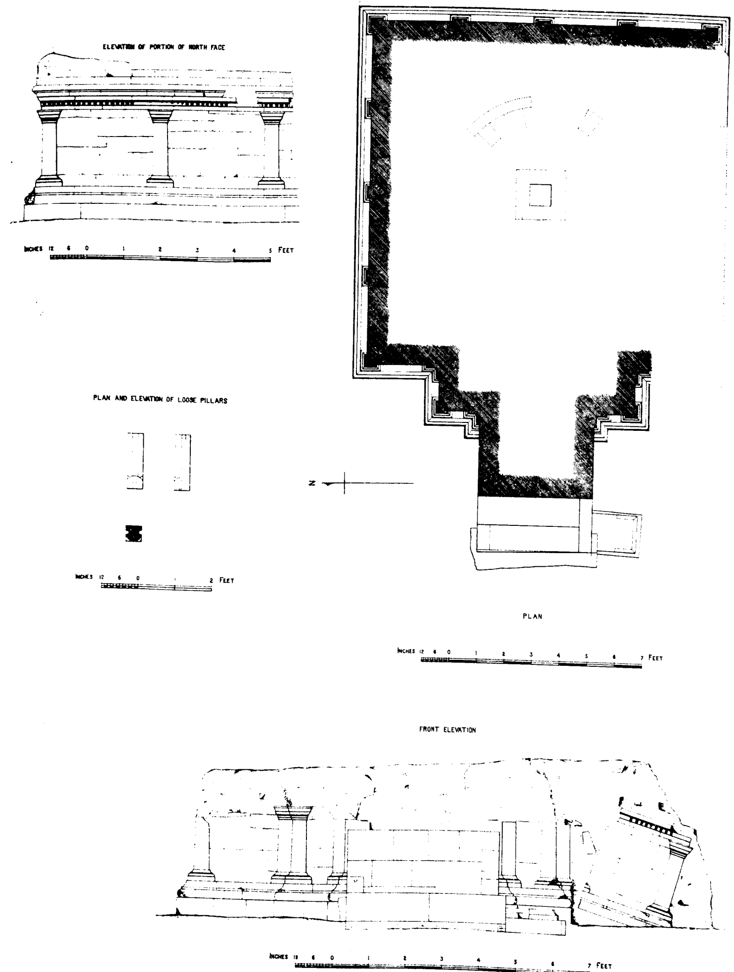
SIRKAP: PLAN AND ELEVATION OF SHRINE II.
