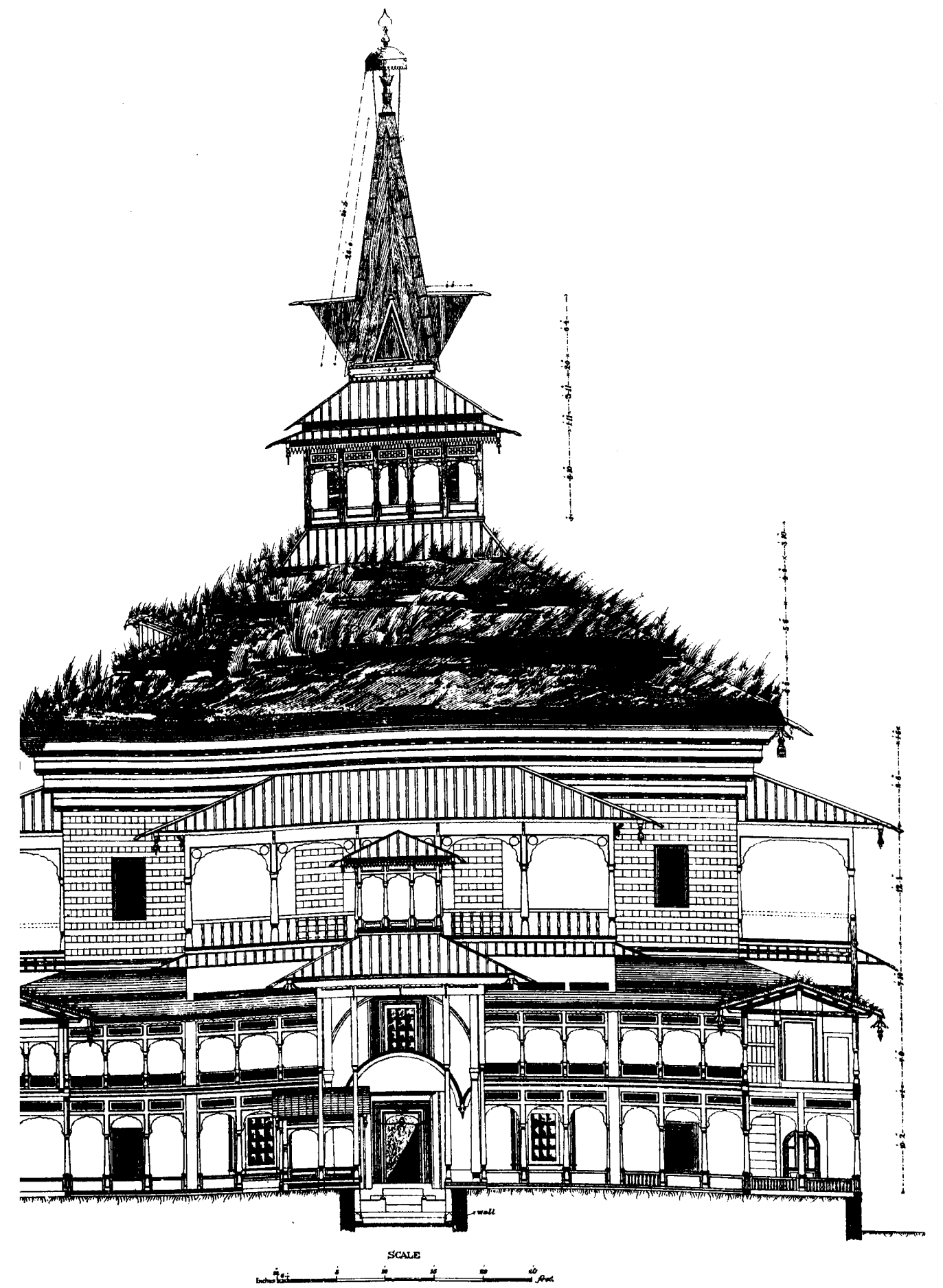
MOSQUE OF SHAH HAMADAN: MAIN ELEVATION.
