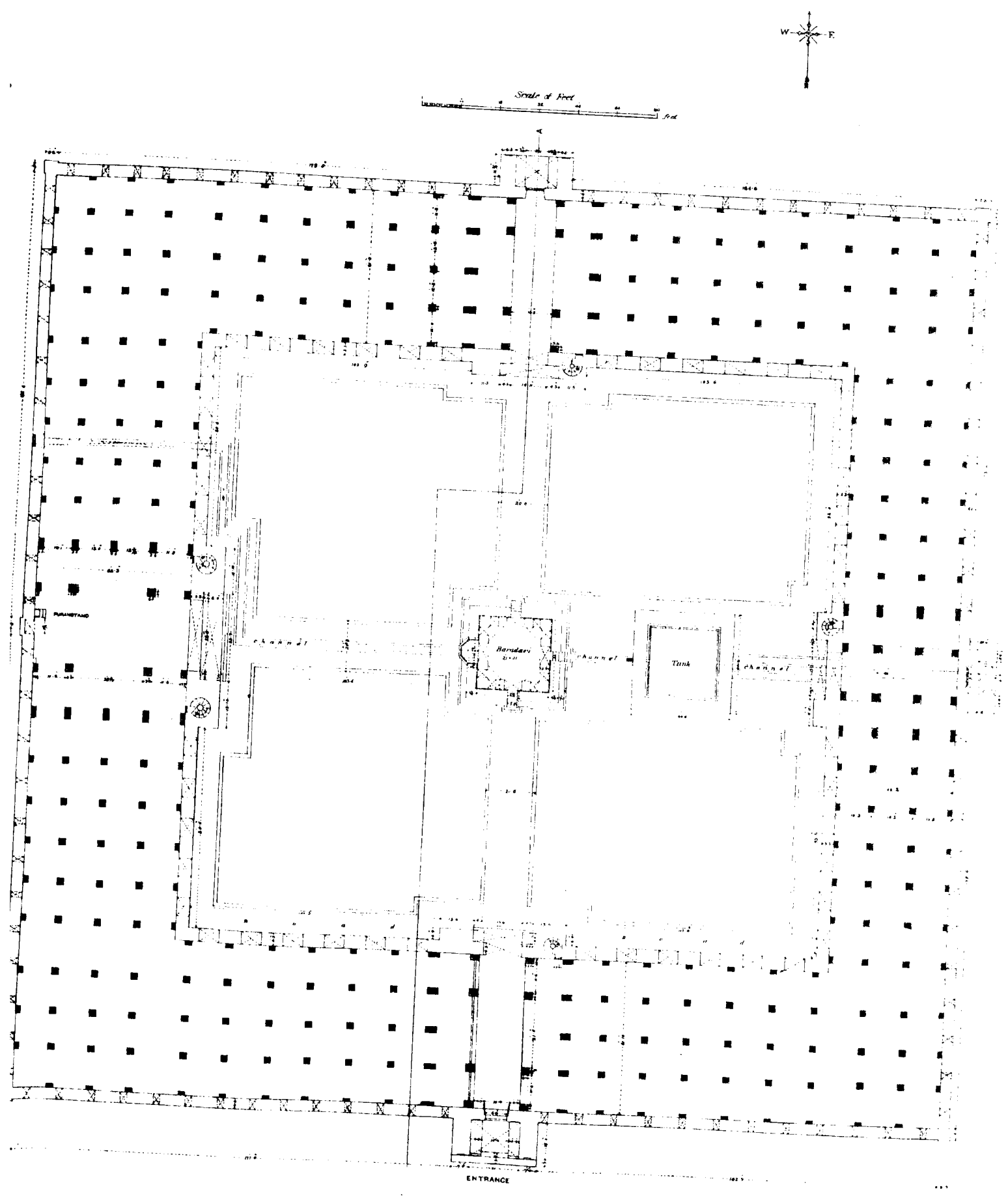
JAMI MASJID: GROUND PLAN.
