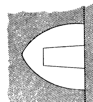
SITAMARHI CAVE 10 Feet = 1 Inch.
