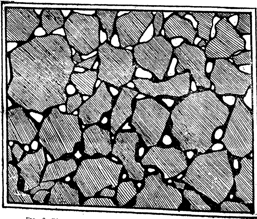
FIG. 28—Diagram to show pore space in soils. The black represents water; the white, air. The soil at the lower edge of the diagram is waterlogged.
