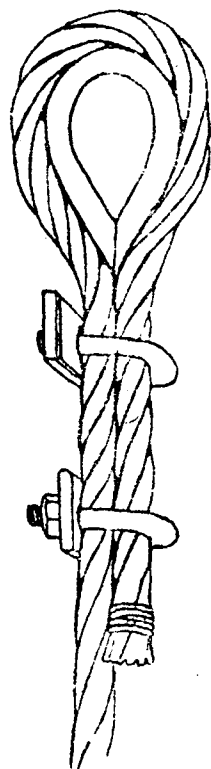
FIG. 9—Method of making loop in steel rope.
