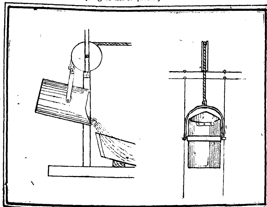
FIG. 8—Tilting bucket as suggested in Stoney's lift.
