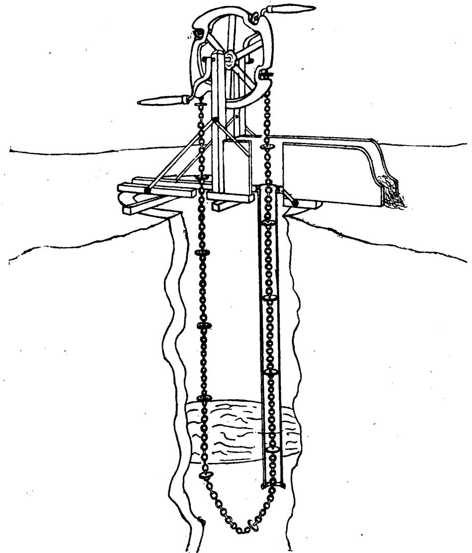
Fig. 16—Chain pump : the circular leather washers fit against the sides of the pipe and push the water up and out into the trough at the surface.
