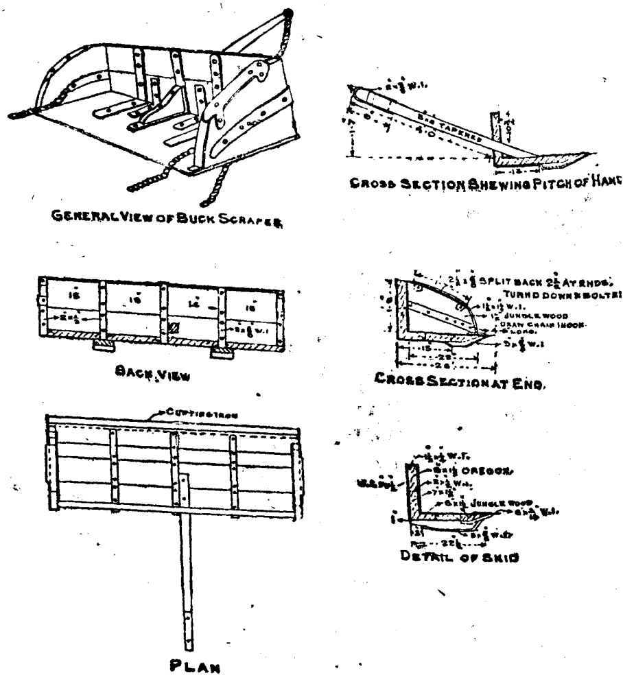
FIG. 24—A buckscraper or levelling board.
