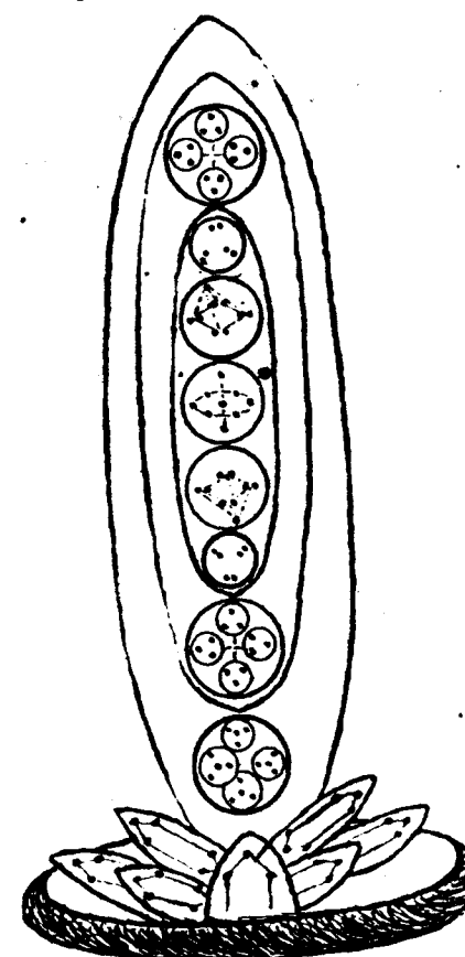
Lithium 127
