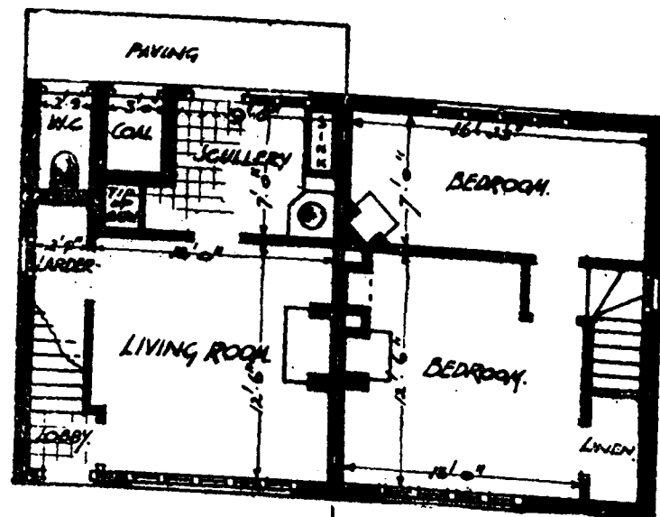
HALF GROUND FIRST FLOOR PLANS.
