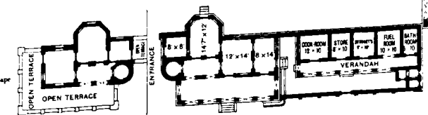
HALF FIRST HALF GROUND FLOOR PLAN DACC
