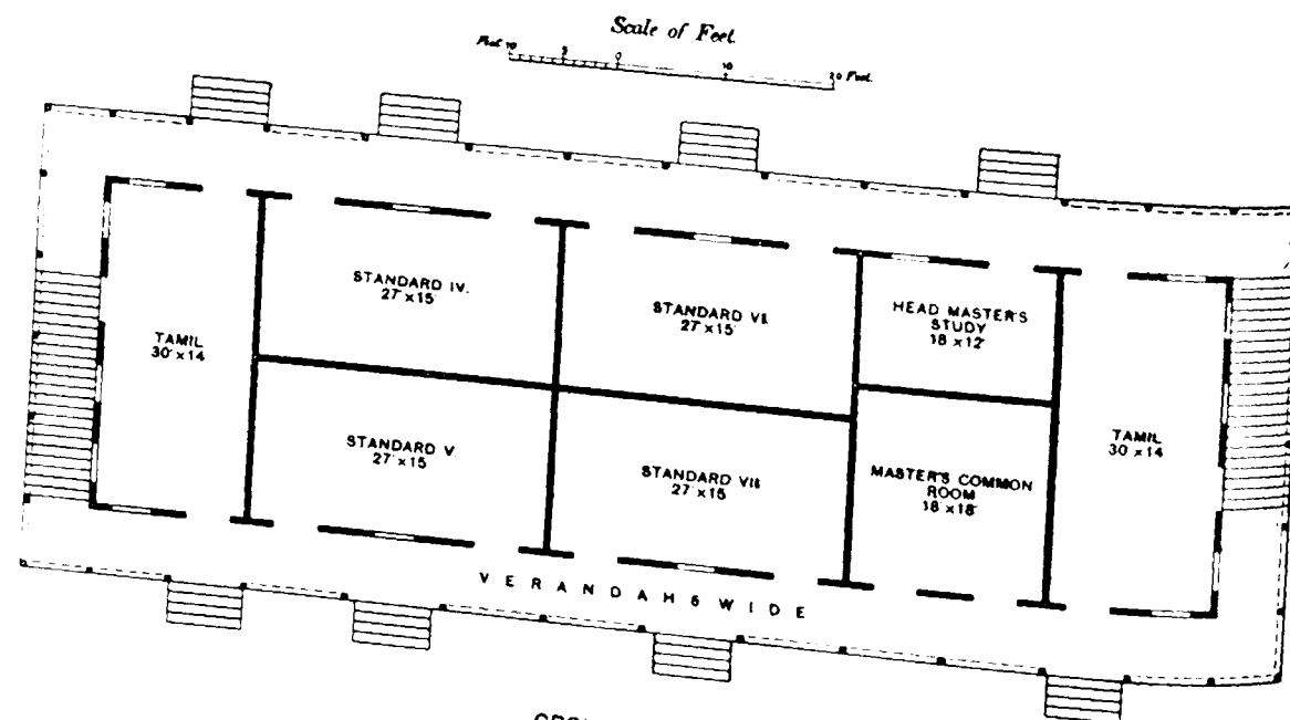
GROUND FLOOR. GOVERNMENT ANGLO-VERNACULAR MIDDLE SCHOOL, MAYMYO.
