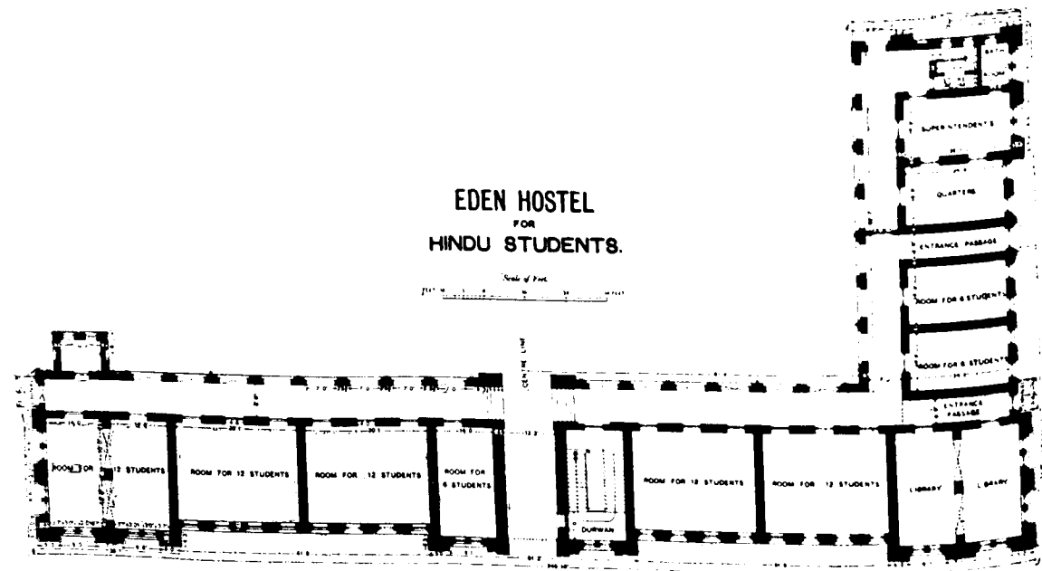
PLAN OF GROUND FLOOR NORTH AND WEST SIDES.
