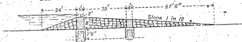
FIG. 2.—CROSS SECTION DEHRI WEIR ON SONE RIVER.
