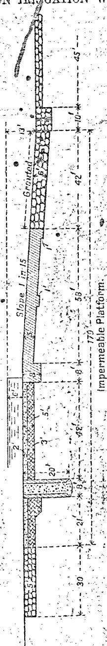
PLATE V.—CROSS SECTION KILANKI WEIR ON CHENAB RIVER.
