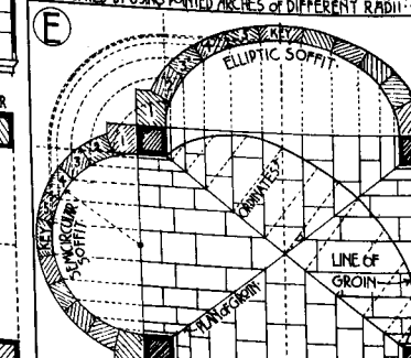
RENAISSANCE CROSS VAULT. OBLONG COMPARTMENT & INTERSECTING VAULTS OF UNEQUAL SPAN BUT EQUAL HEIGHT OBTAINED BY USE OF ORDINATES. GROIN LINE STRAIGHT ON PLAN.
