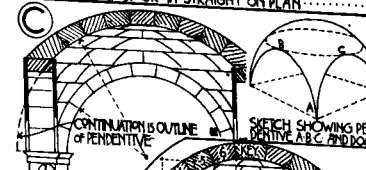
SECTION OF EARLY TYPE PENDENTIVE PART OF DOME.
