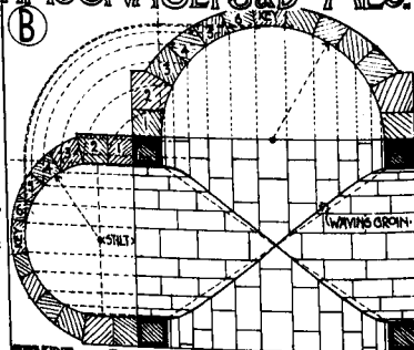
TYPE OF ROMANESQUE CROSS VAULT. OBLONG COMPARTMENT & SEMI-CIRCULAR VAULTS OF UNEQUAL SPAN. THE LESSER VAULT SLANTED MAKING LINE OF GROIN WAVY.
