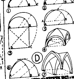
EARLIEST SEMI-GROINED VAULT.
