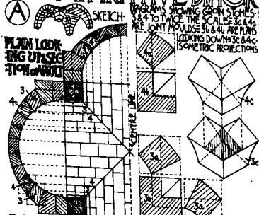
ROMAN CROSS VAULT. THE COMPARTMENT IS SQUARE, AND SEMI-CIRCULAR VAULTS OF EQUAL HEIGHT... NOTING THE LINE OF GROIN STRAIGHT ON PLAN.
