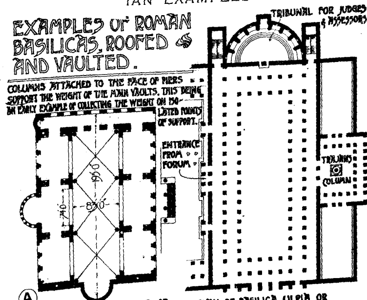
(B) PLAN OF BASILICA ULPIA OR TRAIANUS BASILICA, A.D. 98.
