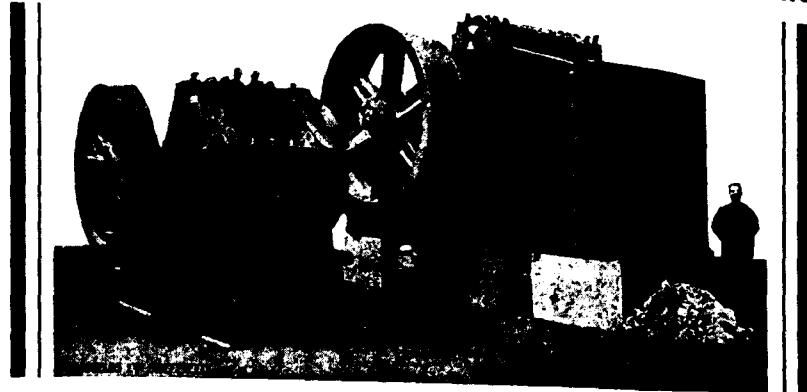
HADFIELDS ALL STEEL SLEDGING BREAKERS 36" x 24" MACHINE - - OUTPUT 80 TONS AN HOUR 54" x 42" MACHINE - - OUTPUT 200 TONS AN HOUR
