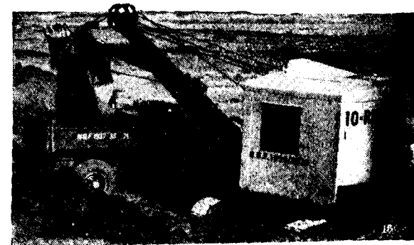
A Ruston-Bucyrus 10-RB \frac{3}{8} yard Diesel Shovel working on the Johannesburg-Durban National Road—one of over 60 10-RB excavators sold to South Africa for development work.
