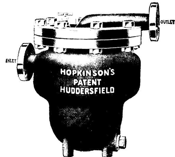
Hopkinson's Patent "Duplus" Steam Trap.
