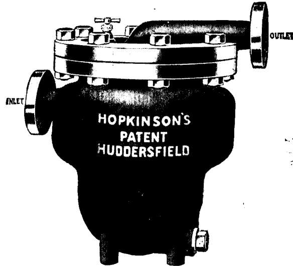
Hopkinsons' Patent "Duplus" Steam Trap.
