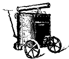
"PHENIX RAPID" Tar and Pitch Boiler.
