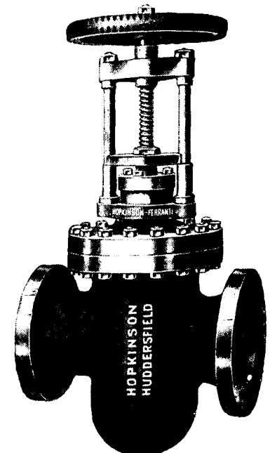
HOPKINSON-FERRANTI PATENT STEAM STOP VALVE
