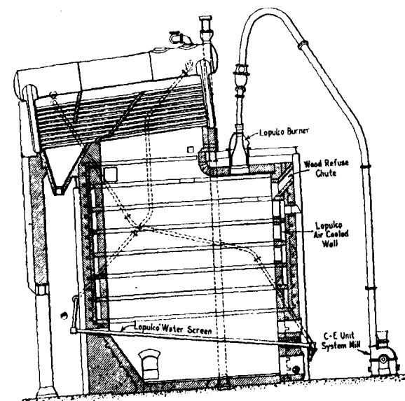
Water Tube Boiler installed with the Lopulco Combustion Chamber and Unit System of Firing.
