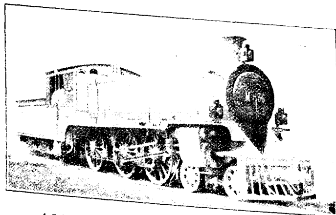
4-6-0 Tender Engine for the Indian State Railways.
