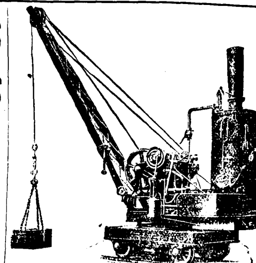
LOCOMOTIVE STEAM CRANE. (Fig. 758)
