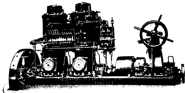
66 B.H.P. MARINE OIL ENGINE, GEAR REVERSE TYPE.
