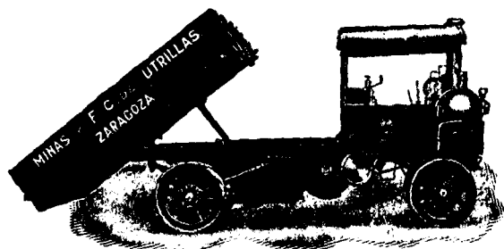
Tipping Wagon with Patent Mechanically-operated Tipping Gear.
